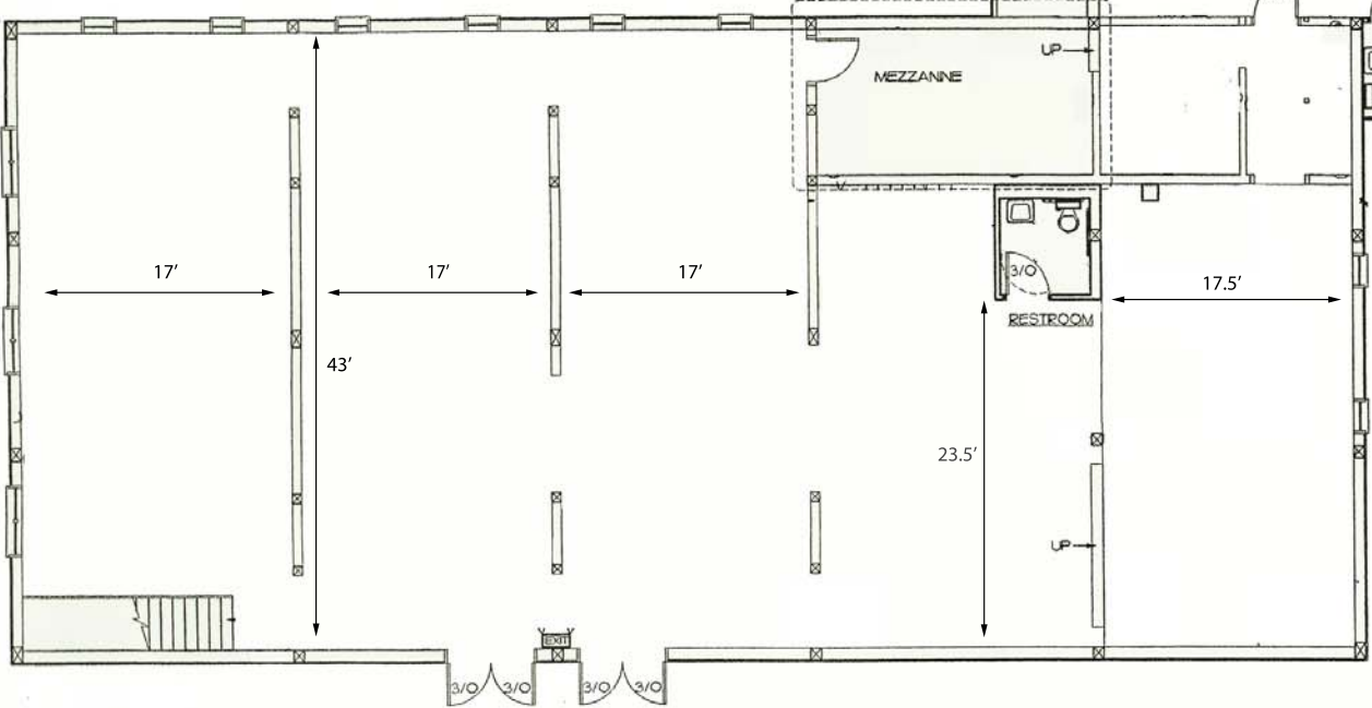
MAIN LEVEL FLOOR PLAN
